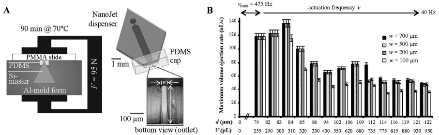
Figure 3. (A) The flexible fabrication process of the disposable phase-gap cap. (B) Maximum volume ejection rates where no flooding of the phase-gap occurs.
